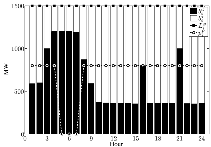
Figure 11. Aggregated economic dispatch of the two BCs between the thermal units and the GPU for study case (a). Exercised VPP energy is also shown.
