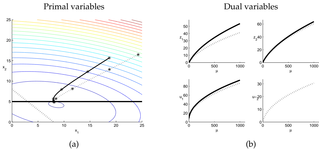
Figure 1: Change in the central path when a new constraint is introduced (dotted line)
